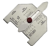
143- AUTOMATIC WELDING GAUGE
